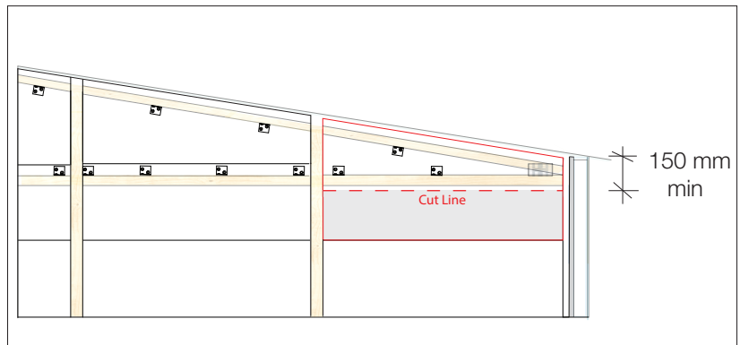
Detail for Low Pitch Skillion Roof
