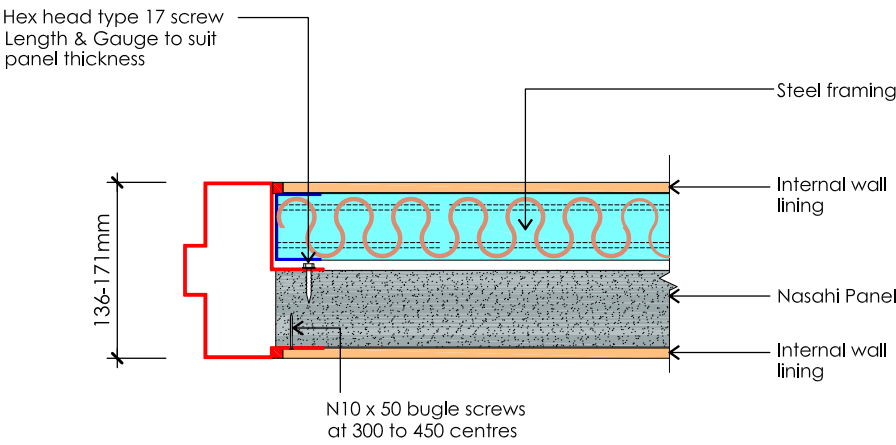
DETAIL 9.0 - FIRE DOOR IN-LINE WITH WALL
