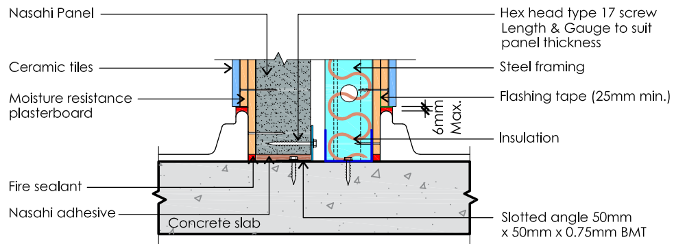
DETAIL 10.0 - BATH/SHOWER AREA
