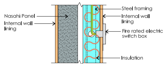
DETAIL 7.1 - POWER SWITCH INSTALLATION TO STEEL STUD / FURRING CHANNEL DETAIL
