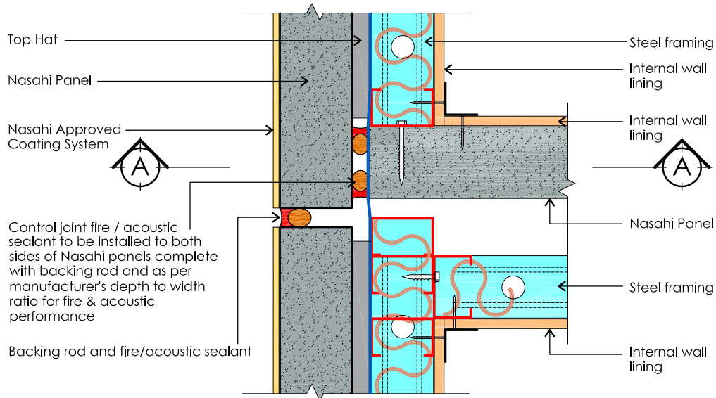
DETAIL 11.0 SYSTEM 1 TO EXTERNAL FACADE WALL JUNCTION
