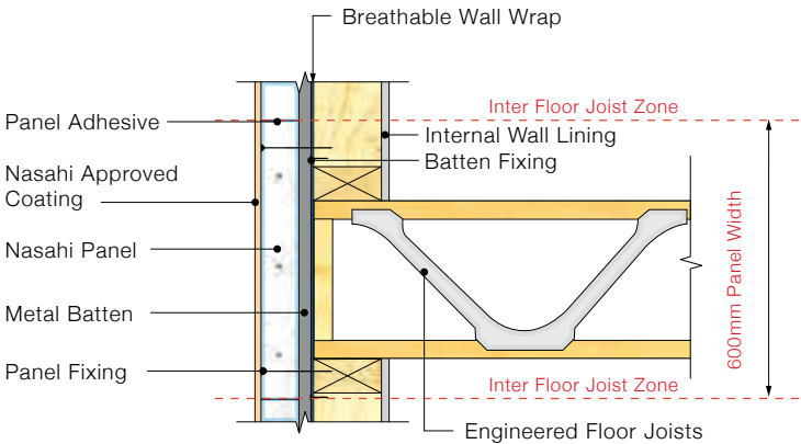
DETAIL 6.2 - Inter Floor Junction (No Panel Joint in Joist Zone)
