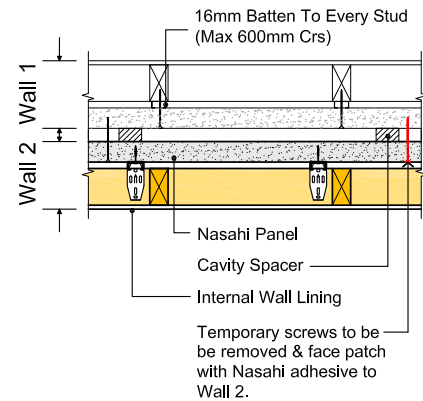
DETAIL 12.3 - Boundary Wall Fixing Detail C
