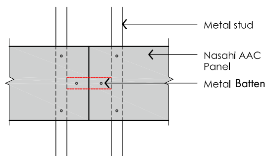
DETAIL 11.2 - Back Blocking for Misaligned Panel (Only for aesthetic purposes, so panels are aligned & flush)
