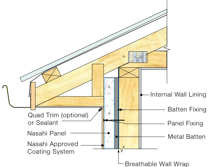
DETAIL 4.3 - Eave Detail (Panel Flush With Lining)
