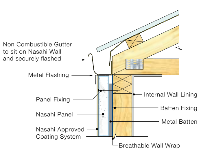
Detail 4.1A - Gutter on Boundary Wall
