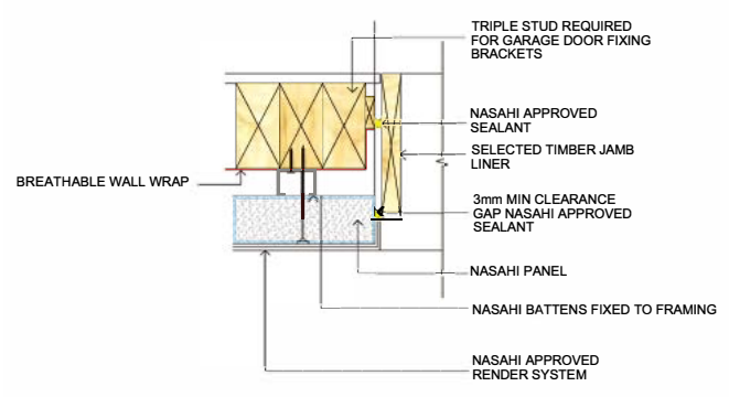
DETAIL 3.6 - Garage Door Jamb Detail
