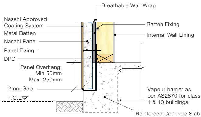
DETAIL 1.1 - Slab Edge Detail (Rebate)
