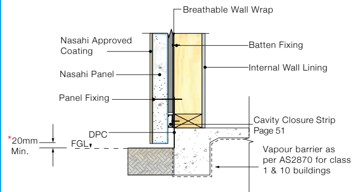
DETAIL 1.2 - Slab Edge Detail (Overhanging)
