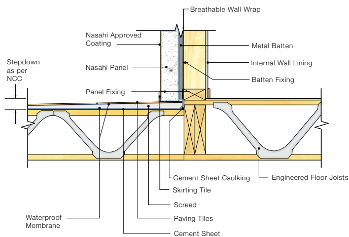
DETAIL 1.4 - Balcony Detail (Timber Frame)
